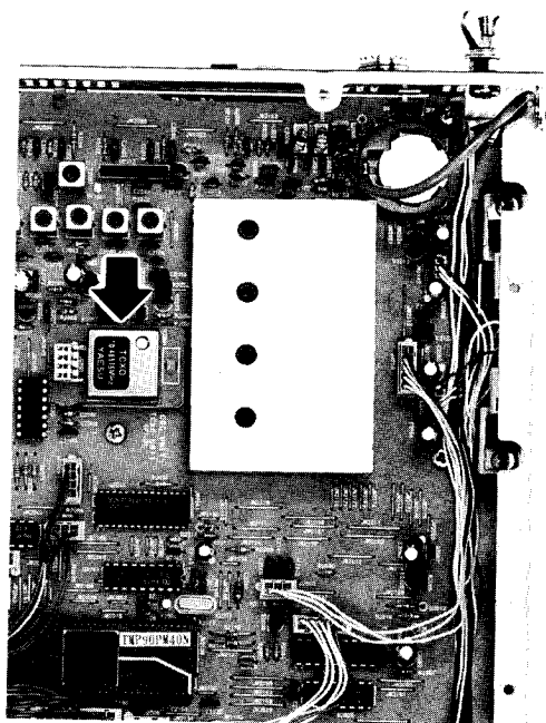
Figure 8: TCXO Installation
