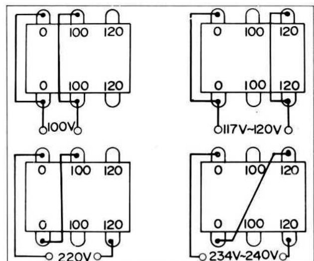
Fig.1 Transformer Primary Wiring
